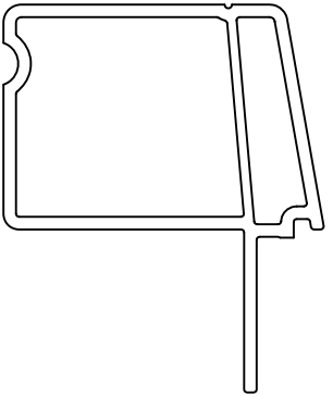
#4566 Moulure 1 3/8"
